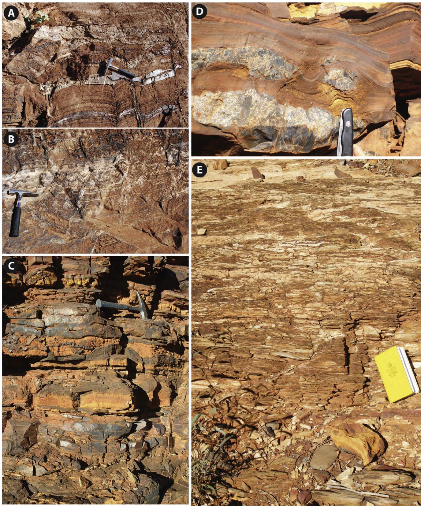
Fig. 4. (A) Low-relief domal precipitates, section B; (B) conical precipitates, section B; (C) early diagenetic chert nodule in iron formation, section C; (D) ironstone within section C; and (E) calcite-rich carbonate within iron formation, section C.
