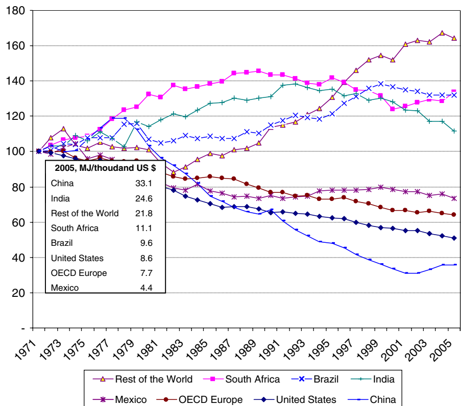
Fig. 2 Primary energy supply per unit of GDP (excluding biomass; MJ/US $2,000 market exchange rate; indexed to 1971, using IEA data)
