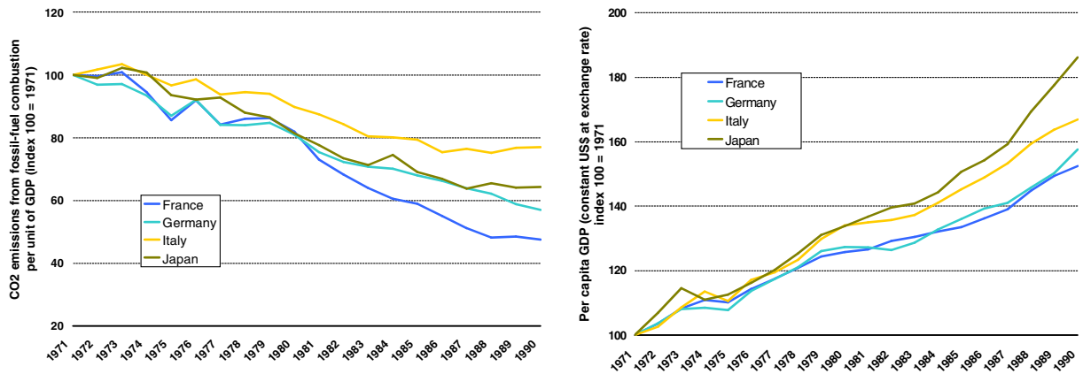
Fig. 1 Left : Evolution of CO 2 emissions from fossil fuel combustion in France, Germany, Italy, and Japan between 1971 and 1990; right : Evolution of GDP per capita in France,
