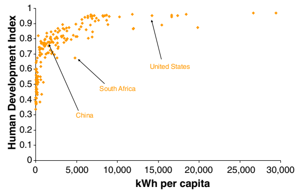
Fig. 3 Human development compared to electricity consumption
