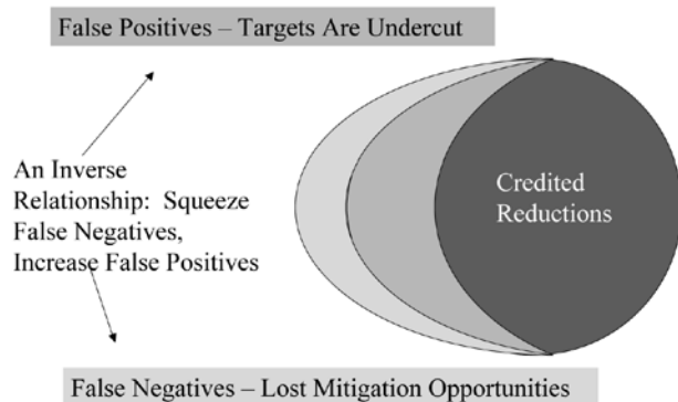
Figure 3b: The Relationship Between False Positives and False Negatives in Additionality Testing
