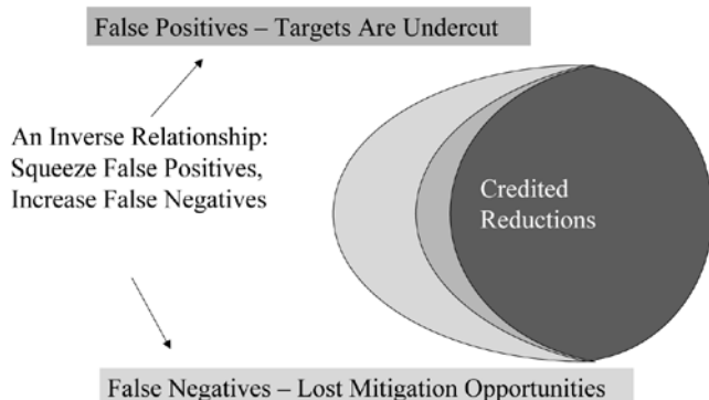
Figure 3b: The Relationship Between False Positives and False Negatives in Additionality Testing
